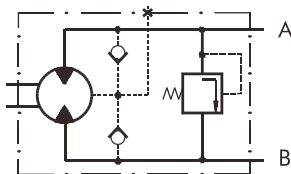
MMP Series with Integrated Internal Crossover Relief Valve A → B, Δp = 100 bar (50 bar)
