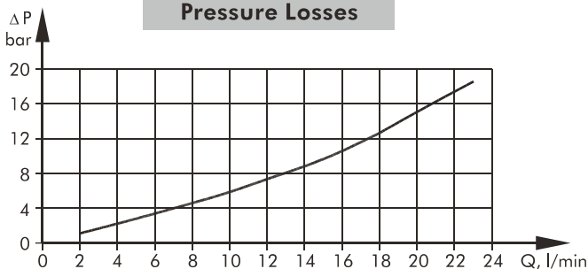
Pressure Losses
